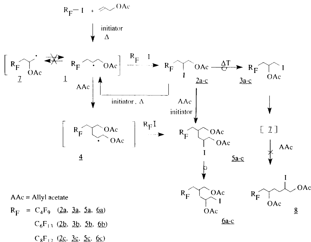
Scheme 1. Reaction mechanism for the radical telomerization of allyl acetate with perfluoroalkyl iodides.
